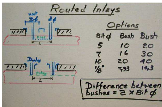
Combinations of guide bush and router bit sizes for Routed Inlays
